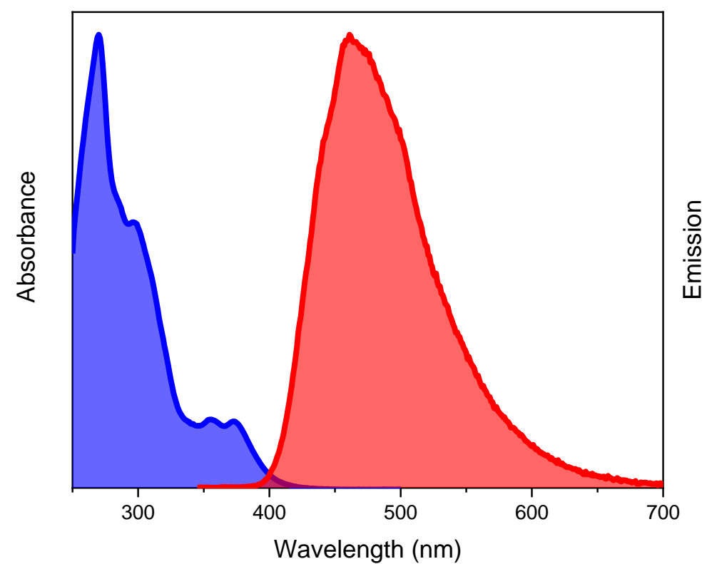
Absorbance and Emission spectra in Ethyl Acetate
