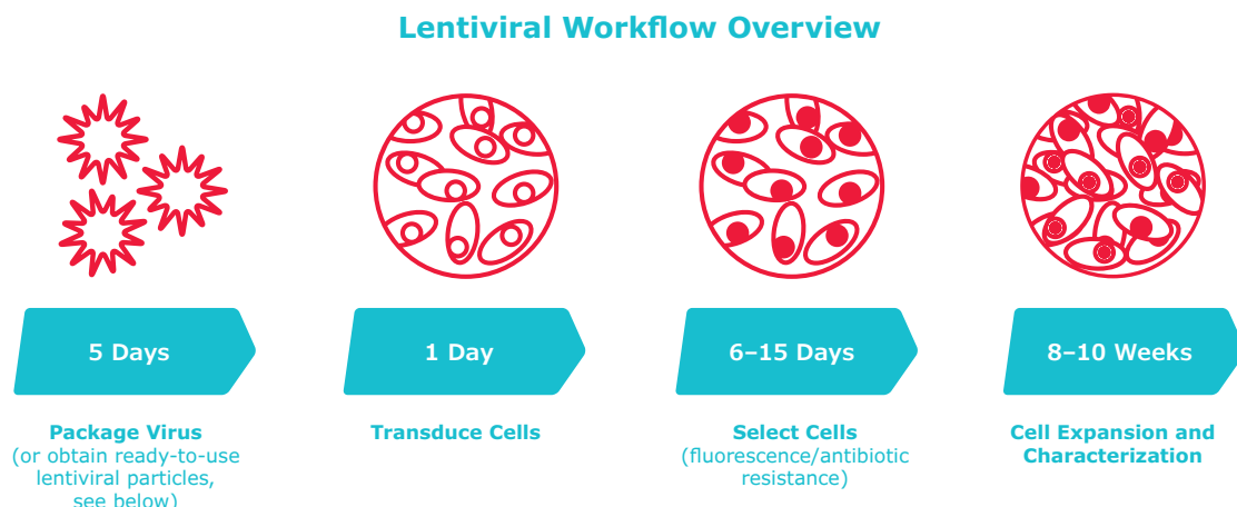
Figure 3: Lentiviral Workflow
