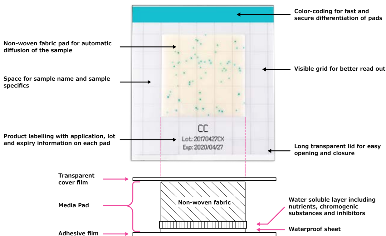
Figure 1: Description of MC-Media Pad®
